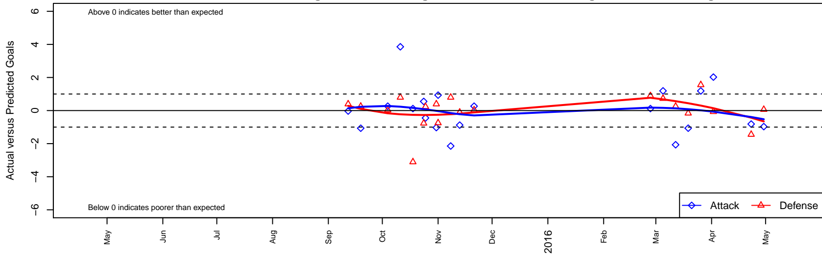
NPSA Titans White G03 Dots are actual minus expected GF (blue circles) and GA (red triangles). Blue line is smoothed change in attack strength. Red is smoothed change in defense strength.
